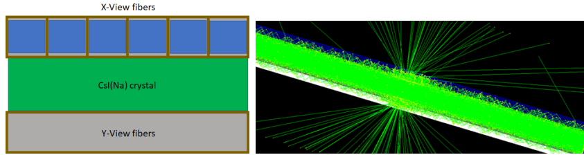
Figure 1. Left panel: Schematic view of the ICC module simulated (not in scale). Right panel: Event display showing the tracks of optical photons produced by a 1 GeV muon crossing the tile at its center. The light yield is reduced of a factor 10 to make the tracks visible.
