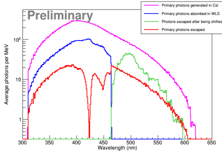
Figure 2. Spectra of all photons tracked by the simulation code. The purple line indicates the primary scintillation photons produced inside the crystal after the muon energy release; the blue line indicates the photons that are absorbed in the any fiber plane; the red line indicates primary scintillation photons escaping outside the ICC; the green line indicates photons escaping outside the ICC after being absorbed and re-emitted by the WLS fibers.
