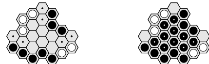
Figure 9: A 4-cycle of alternating consecutively crowding groups with an interior Black virtual connection (left). By Thm. 2, Black captures the region (right).
