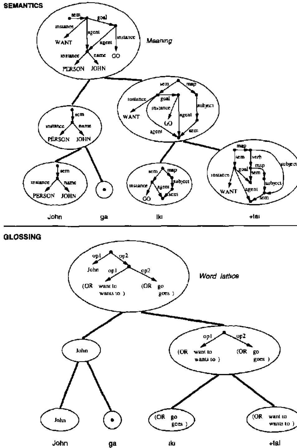
Figure 1 Semantic analysis versus glossing. Both convert parse trees into feature structures using unification-based compositional techniques. Semantics computes a conceptual representation while glossing computes a target language word lattice.
