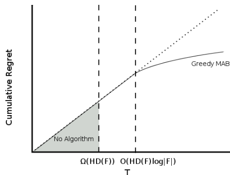
Figure 1: A graphical summary of the main results of this paper. This figure illustrates that any MAB algorithm for a function class \mathcal{F} must suffer linear regret for a number of rounds on the order of the haystack dimension (denoted \text{HD}(\mathcal{F}) ), while the MAB algorithm presented in this paper, called Greedy MAB, begins to suffer sublinear regret after roughly \text{HD}(\mathcal{F}) \log |\mathcal{F}| rounds.
