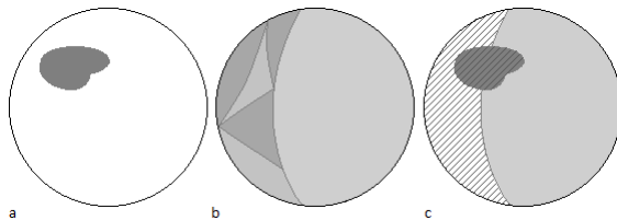
Figure 2: (a) The shaded region represents the subset of functions which attain a maximum at some input x . (b) Querying x also induces a partition of the function space, in which each piece of the partition contains functions that output the same value on x . The least informative query response is thus the largest piece of this partition. (c) Upon querying x , the greedy algorithm eliminates from its attention space a set at least the size of the striped region. This region is the union of the maximizing set and the complement of the largest partition piece.
