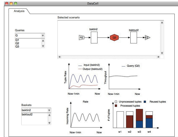
Figure 3: Analyzing performance.
