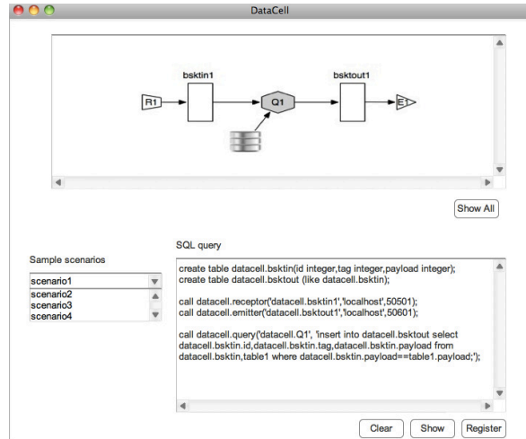
Figure 4: Posing queries.
