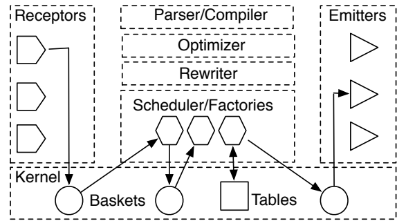
Figure 1: The DataCell architecture.
