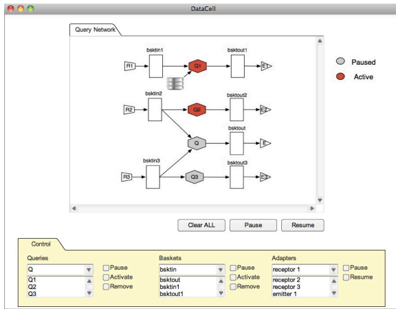
Figure 2: The network of continuous queries.
