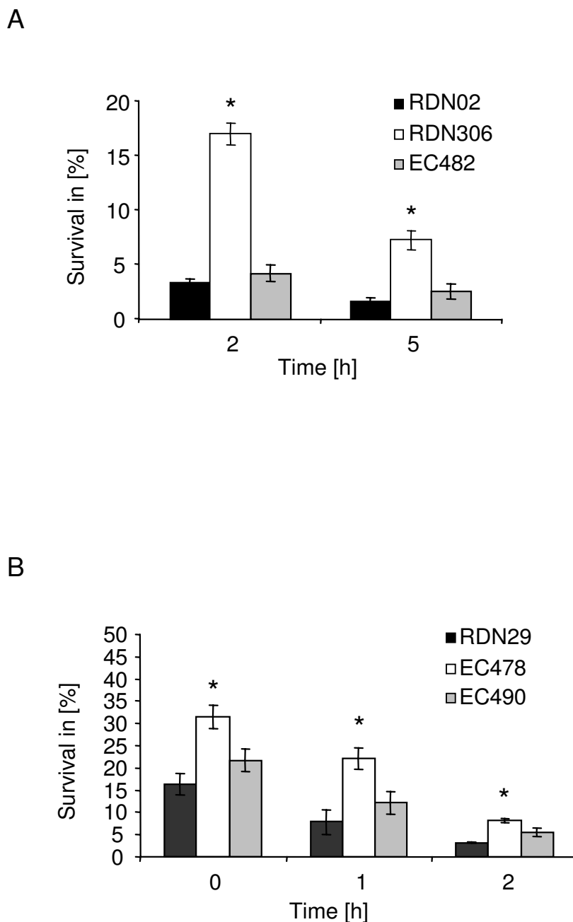
Figure 5 Internalization assays of S. pyogenes in epithelial cells and macrophages. RDN29 (wild-type strain), EC478 (isogenic luxS -deficient mutant) and EC490 (RDN29 (pEC85)); RDN02 (wild-type strain), RDN306 (isogenic luxS -deficient mutant) and EC482 (RDN29 (pEC85)). Bacterial cultures were used to infect (A) HEP-2 human pharyngeal epithelial cells and (B) RAW 264.7 macrophages in an antibiotic protection assay. For this, bacterial cultures were grown to mid-logarithmic (RAW 264.7) and late-logarithmic (HEP-2) phases, growth time points showing optimal internalization rates in RAW 264.7 and HEP-2, respectively. The percent intracellular invasion represents the average CFU/ml number of viable intracellular bacteria recovered at different times following addition of antibiotics versus the average CFU/ml number of inoculated bacteria \times 100 . The average values and standard deviations of three independent assays are shown. The asterisks indicate that the differences in survival rates between the luxS -deficient mutants and the wild-type strains were statistically significant ( P < 0.01 for Hep-2 epithelial cells, P < 0.05 for RAW 264.7 macrophages). Similar data were obtained for both M1 and M19 serotypes.
