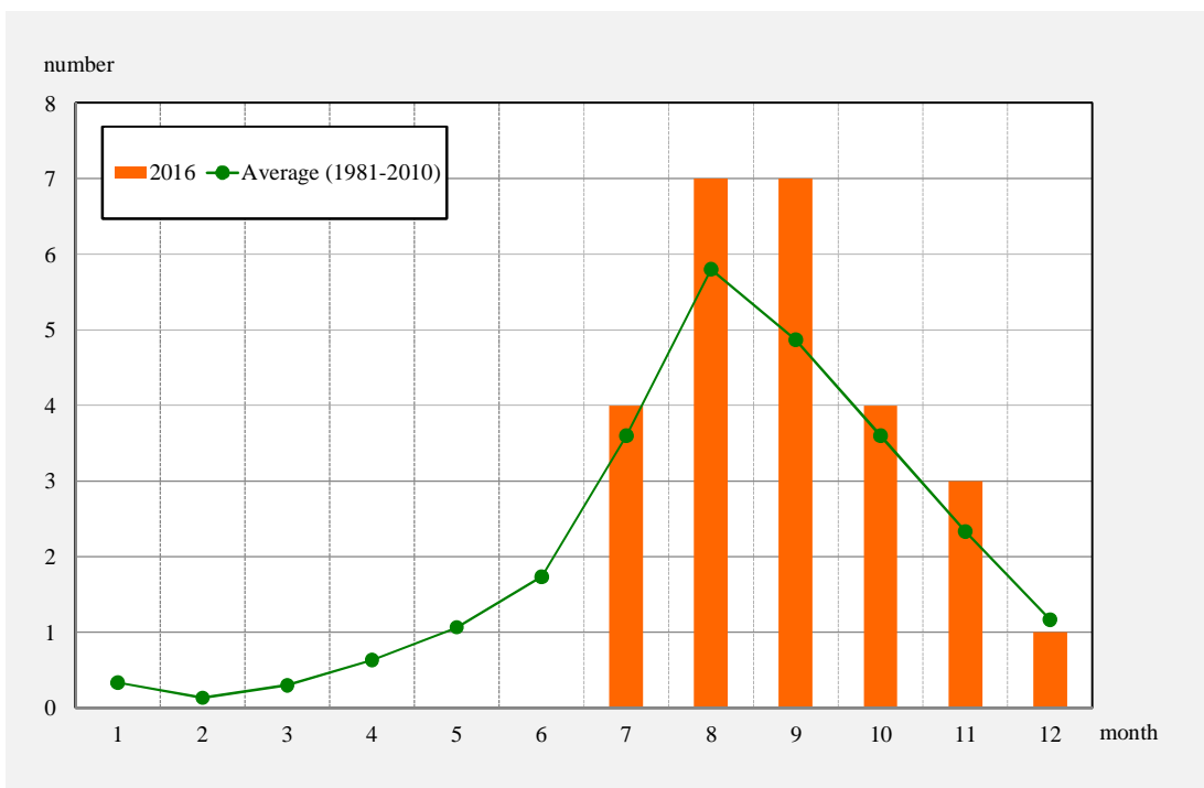
Figure 3.2 Monthly number of TC formations for 2016 compared to the climatological normal
