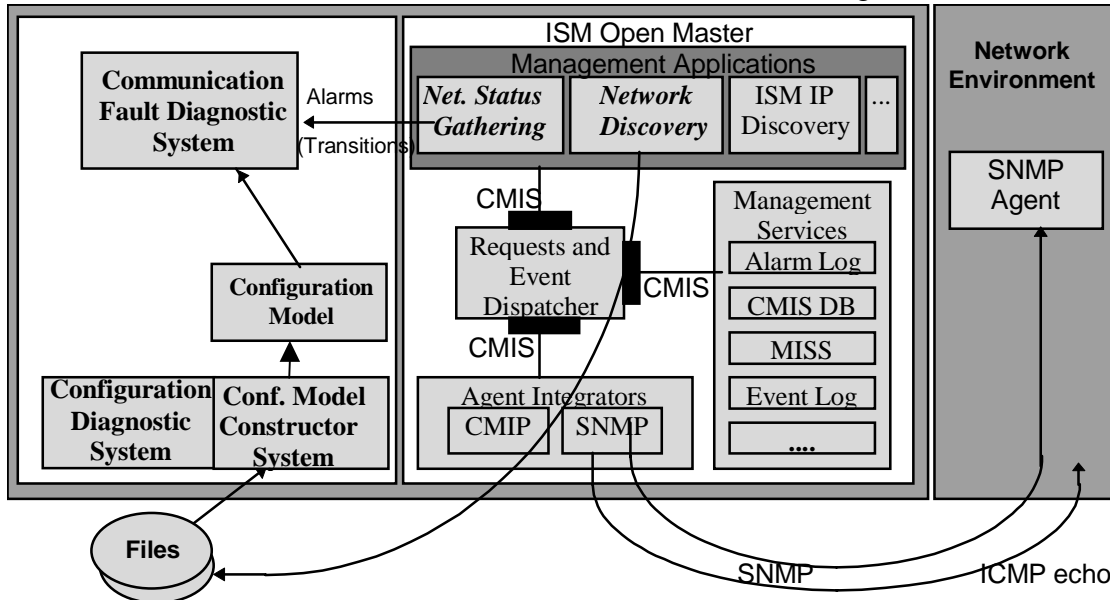
Figure 5. System Architecture.
