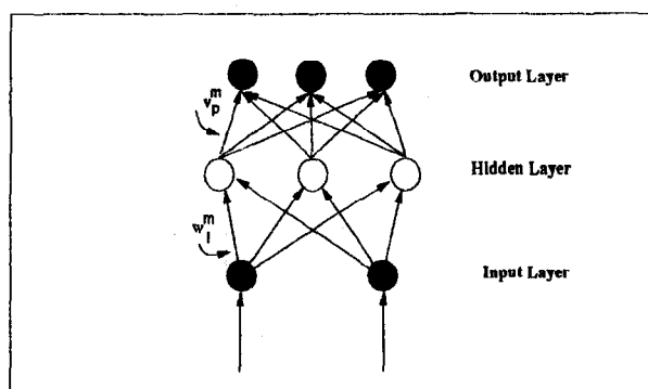
Figure 1: A three layer feedforward neural network.
