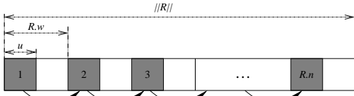
Figure 1: Single Sequential Traversal: s\_tra(R, u)
