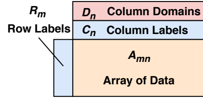
Figure 3: The Dataframe Data Model
