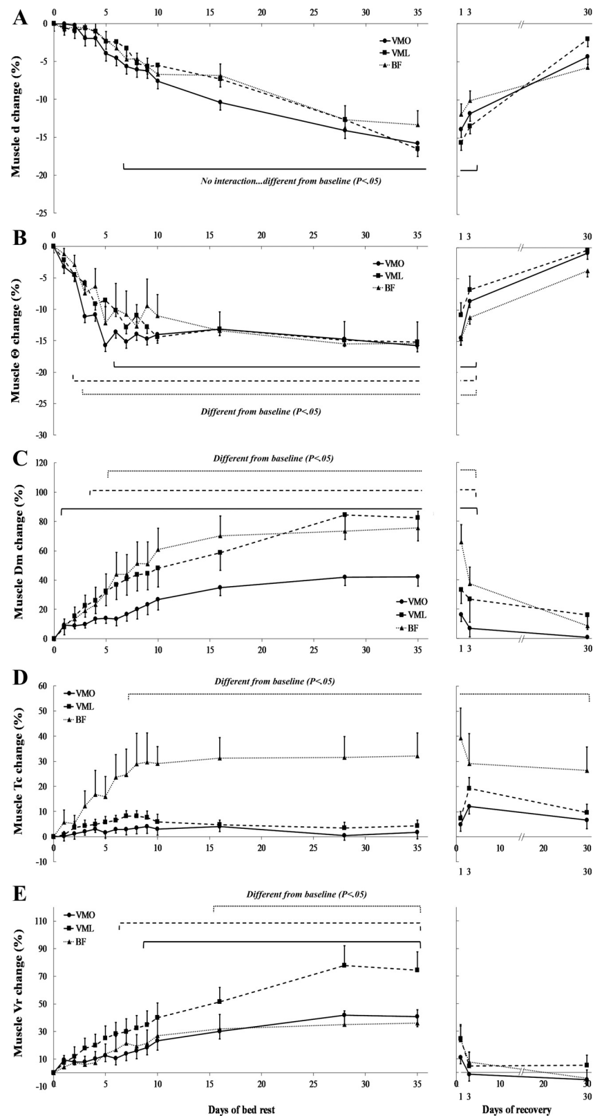
Fig. 2. Changes in (A) thickness (d), (B) pennation angle ( \theta ), (C) tensiomyographic displacement (Dm), (D) contraction time (Tc), and (E) velocity of radial displacement ( V_r ) during 35-day bed rest and 30-day recovery in the vastus medialis oblique (VMO), vastus medialis longus (VML), and biceps femoris (BF). Values are means \pm SE.
