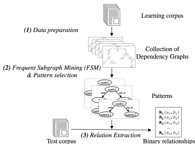
Fig. 2: Overview of our Relation Extraction (RE) method
