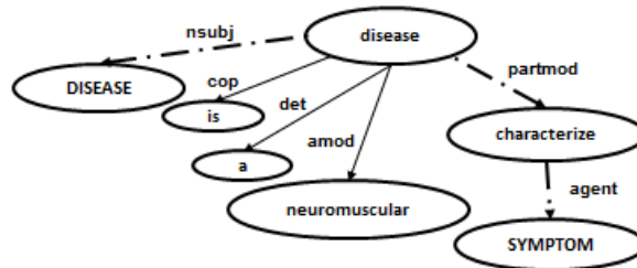
Fig. 7: The shortest path between DISEASE and SYMPTOM
