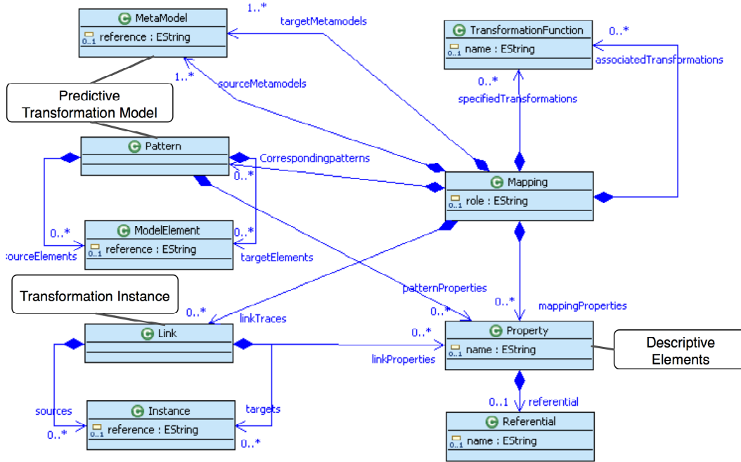
Figure 4. A Mapping MetaModel. Containment relations between Mapping and Metamodels are due to the Eclipse Modeling Framework needs.
