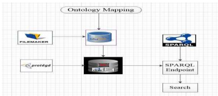
Fig. 3. Design Scenario of Buddha Ontology
