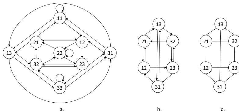
Figure 1: For \Sigma = \{1, 2, 3\} we show: (a) the directed de Bruijn graph cDB((\sigma, \cdot)1, 2) ; (b) the directed Kautz graph cDB(\sigma, 2, 2) ; (c) the undirected Kautz graph cDB^u(\sigma, 2, 2) .
