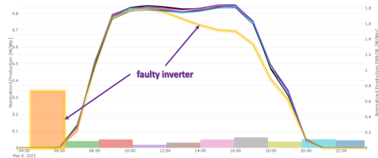
Figure 4: A single day of PV Power production (scaled to Inverter Nominal Power) as continuous lines and the relative model predictions as dotted lines. Highlighted a single faulty inverter showing a transient power loss. The bar plot of the model prediction error for each inverter allows to easily recognize the faulty one by applying a threshold.
