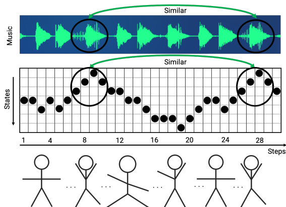
Figure 1: Given input music (top), we generate an aligned dance choreography as a sequence of discrete states (middle) which can map to a variety of visualizations (e.g., humanoid stick-figure pose variations, bottom). Video available at https://tinyurl.com/ybfakpfx .
