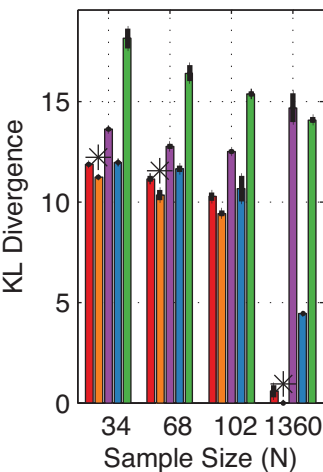
Band ( \kappa = 100 )
