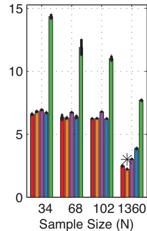
Scale-free ( \kappa = 100 )
