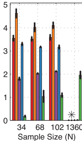
Cluster ( \kappa = 100 )
