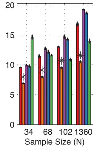
Scale-free ( \kappa = 100 )
