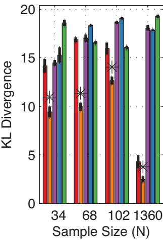
Band ( \kappa = 100 )
