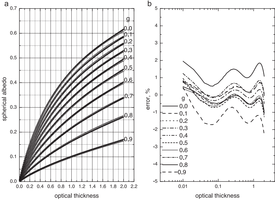
Fig. 1. (a) The spherical albedo as function of optical thickness for the Henyey–Greenstein phase function with various values of g=0.0–0.9 . Crosses give the results of our parameterization, circles are obtained by exact radiative transfer calculations with \omega_0=1 . (b) The relative error of Eq. (3) in % for various values of g .
