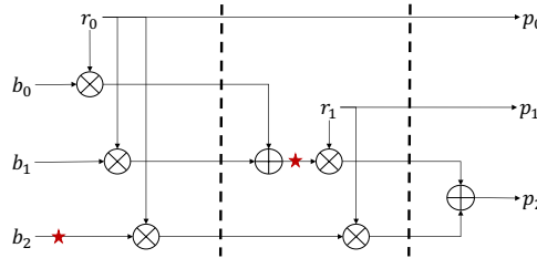
Figure 13: Conversion from Boolean to multiplicative masking with second-order leakage
