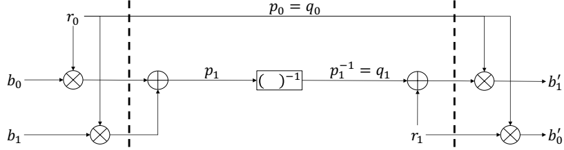
Figure 2: First-order shared implementation of an inversion in \mathbb{F}_q . The dashed lines depict registers.
