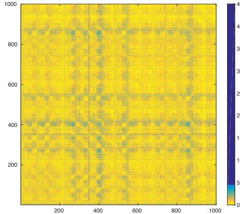
Figure 12: Non-specific bivariate leakage detection test on 15 clock cycles of a second-order protected AES with 50 million traces.
