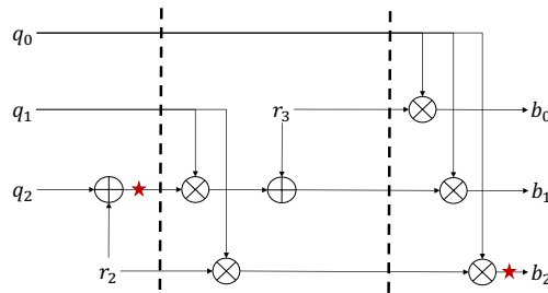
Figure 14: Conversion from multiplicative to Boolean masking with second-order leakage
