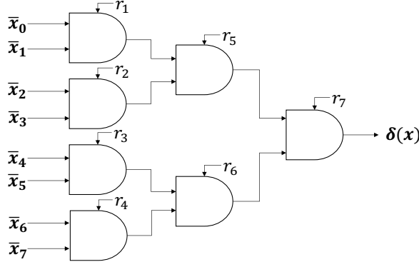
Figure 4: Circuit for the shared Kronecker delta function \delta(\mathbf{x}) for n = 8
