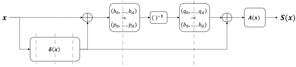
Figure 5: First-order adaptive masking implementation of the AES S-box. The dotted grey lines depict registers.
