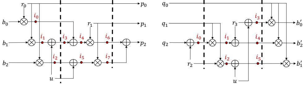
Figure 17: Second-order Boolean to multiplicative (left) and multiplicative to Boolean (right) conversion circuits with intermediate probes
