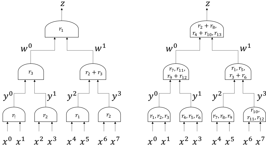
Figure 18: First- (left) and second-order (right) Kronecker Delta. Notation is adapted for clarity.
