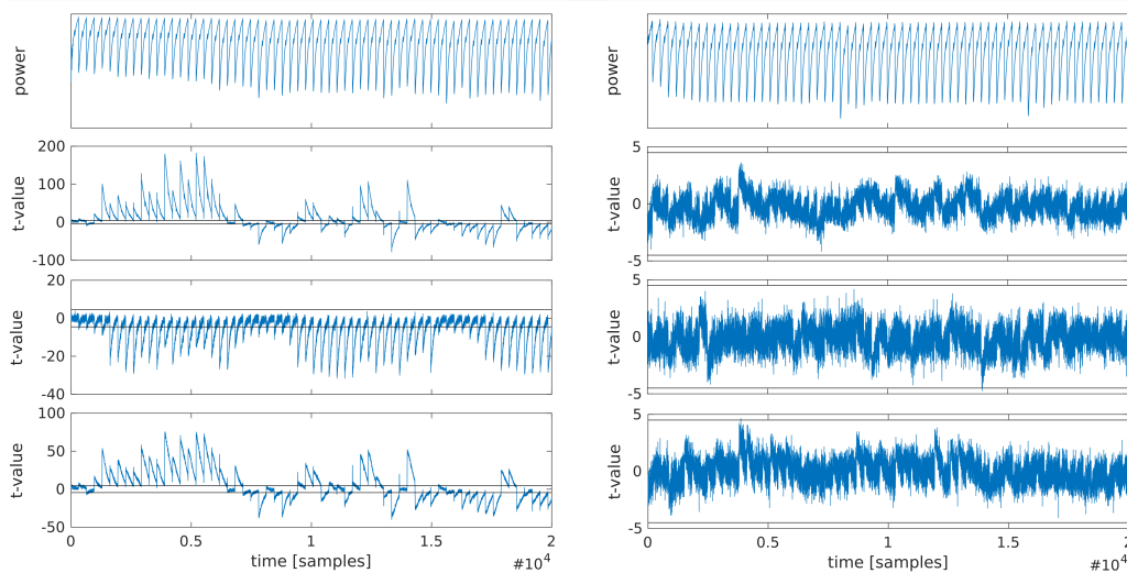
Figure 9: Non-specific leakage detection test on 2.5 rounds of encryption of a second-order protected AES. Left: PRNG off; 12 000 traces. Right: PRNG on; 50 million traces. Rows(top to bottom): exemplary power trace, first-order, second-order, third-order t-value.
