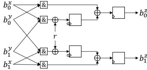
Figure 1: First-order DOM- indep multiplier
