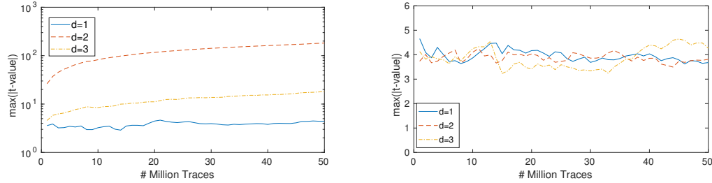
Figure 10: Evolution of the maximum absolute t-value across the measurements. Left: First order. Right: Second order.
