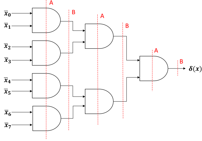
Figure 15: Circuit for the shared Kronecker delta function \delta(x) for n = 8
