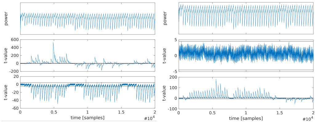
Figure 8: Non-specific leakage detection test on 2.5 rounds of encryption of a first-order protected AES. Left: PRNG off; 12 000 traces. Right: PRNG on; 50 million traces. Rows(top to bottom): exemplary power trace, first-order, second-order t-value.
