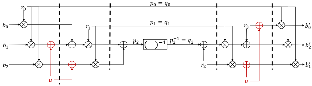
Figure 3: Second-order shared implementation of an inversion in \mathbb{F}_q . The dashed lines depict registers.
