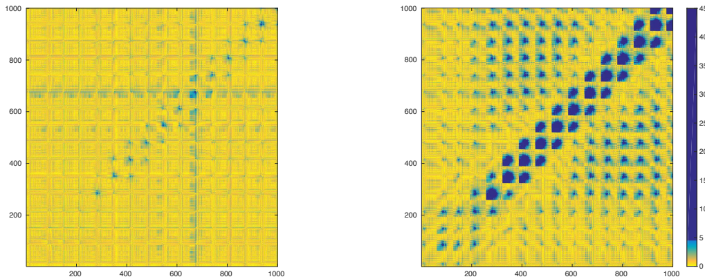
Figure 11: Non-specific bivariate leakage detection test on 15 clock cycles of a first-order protected AES. Left: 1 million traces. Right: 45 million traces.
