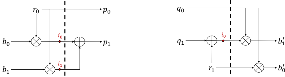
Figure 16: First-order Boolean to multiplicative (left) and multiplicative to Boolean (right) conversion circuits with intermediate probes
