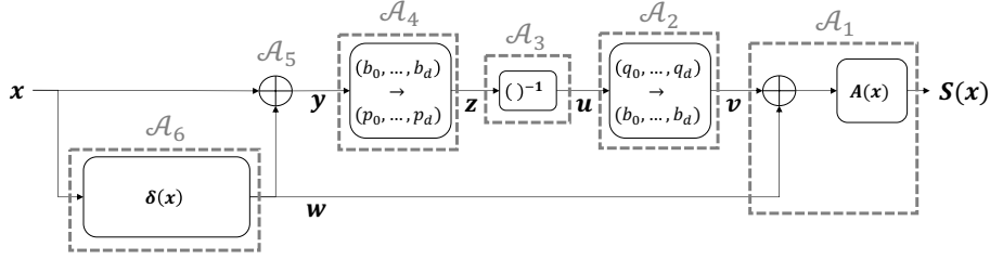
Figure 7: AES S-box
