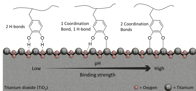
Fig. 9 Binding modes of Dopa to \text{TiO}_2 . This simplified \text{TiO}_2 surface contains titanium atoms (grey) and oxygen atoms (red). The binding mode of Dopa to \text{TiO}_2 is pH dependent with bidentate H-bonding favored below pH 5.5, monodentate H-bonding combined with one coordination bond favored at intermediate pH, and two coordination bonds favored at pH above 7.0. Fig. 9 adapted from [61].
