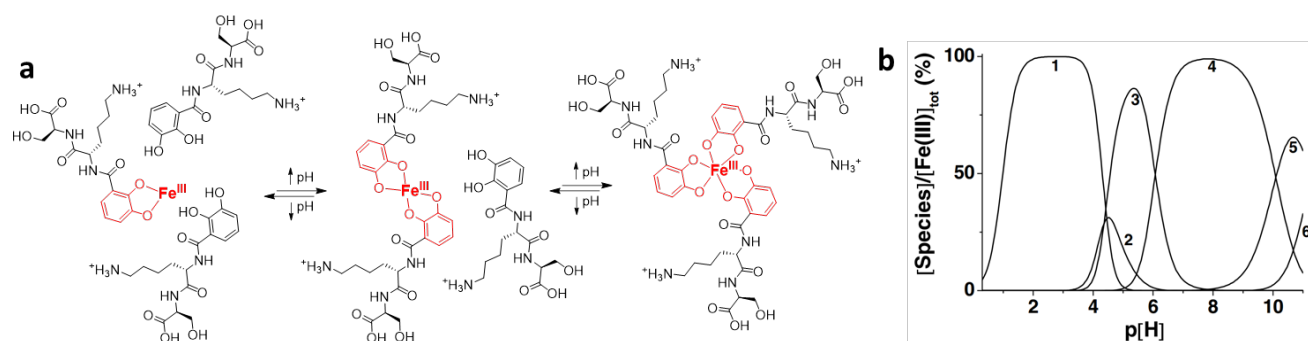
Fig. 3 pH Dependence of Fe(III) Coordination by the Catechol in Chrysobactin. a Mono-catechol complexation is favored at low pH and tris-catechol complexation favored at high pH.
