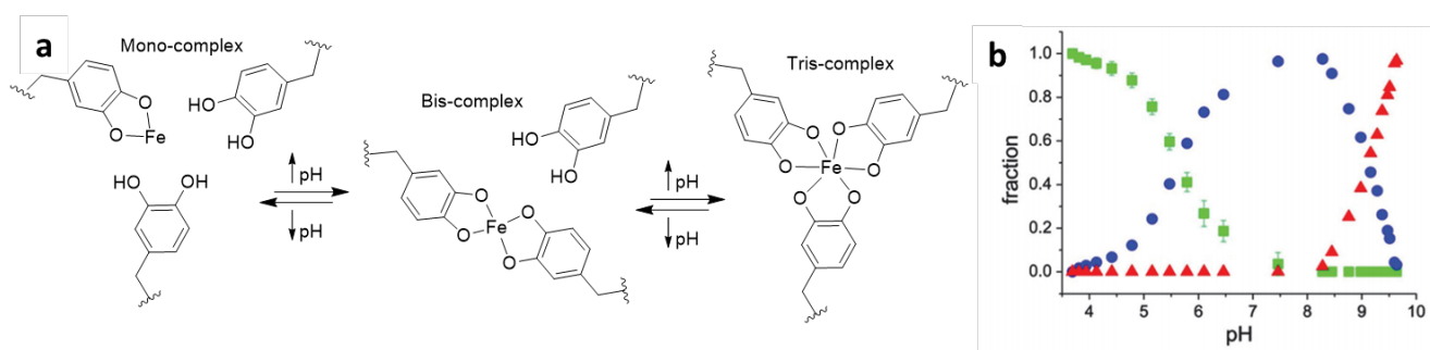
Fig. 4 Fe(III) Coordination to DOPA. a Fe(III)-DOPA coordination is pH-dependent, with mono-complexation favored at low pH and tris-complexation favored at high pH. b Dopa-modified polyethylene glycol (PEG-Dopa 4 , 10 kDa PEG core) in solution with FeCl 3 (Dopa:Fe(III) ratio = 3:1) shows a pH dependence in the relative fraction of mono- (green), bis- (blue), and tris-catechol-Fe(III) (red) complexes. Fig. 4 adapted from [26].
