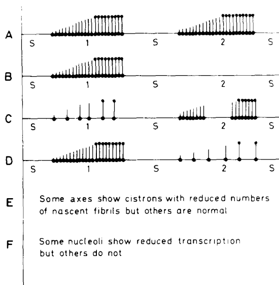
FIGURE 13 Schematic presentation of various alternatives in morphological changes correlated with reduced transcriptions of rDNA. Cistron regions are indicated by the numbers and are separated from each other by spacer intercepts (S). For explanation and discussion, see text.
