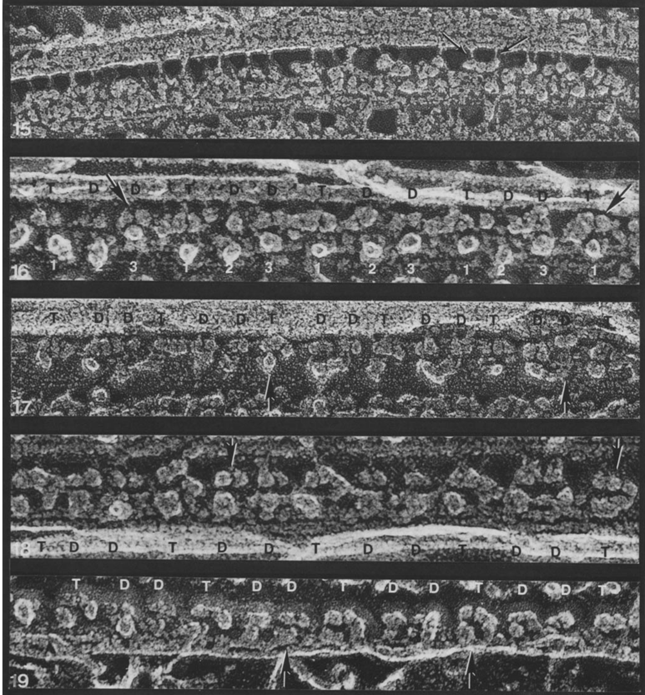
FIGURES 15-19 Rows of inner arms in rigor axonemes. Dyad (two-headed) arms are designated D; triad (three-headed) arms are designated T. Arrows indicate examples in each row whose morphology is particularly well preserved. (Fig. 15) Chlamydomonas pf-14 mutant, showing inner arm stalks (arrows). \times 270,000 . (Figure 16) Ctenophore comb row; spokes S_1 - S_3 are labeled 1-3. The leftmost triad and two rightmost dyads are not well preserved. \times 350,000 . (Figure 17) Sea urchin sperm tail. \times 350,000 . (Figure 18) Sea urchin sperm tail. \times 440,000 . (Figure 19) Ctenophore comb row. \times 440,000 .
