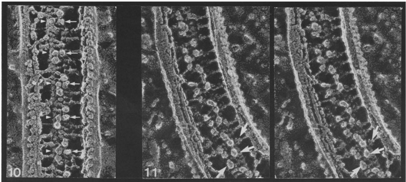
FIGURES 10 and 11 Helical organization of the radial spoke system of Chlamydomonas (Fig. 10) and Tetrahymena (Fig. 11, stereo pair). Adjacent sets of two (Fig. 10) or three (Fig. 11) spokes form a right-handed helix as they ascend around the central pair, with an incremental rise of 32 nm. In Fig. 10, S_1 spokes of the leftward set are indicated by arrowheads, and S_2 spokes of the rightward set are indicated by arrows. In Fig. 11, arrows indicate three successive S_1 heads. (Fig. 10) \times 140,000 ; (Fig. 11) \times 170,000 .
