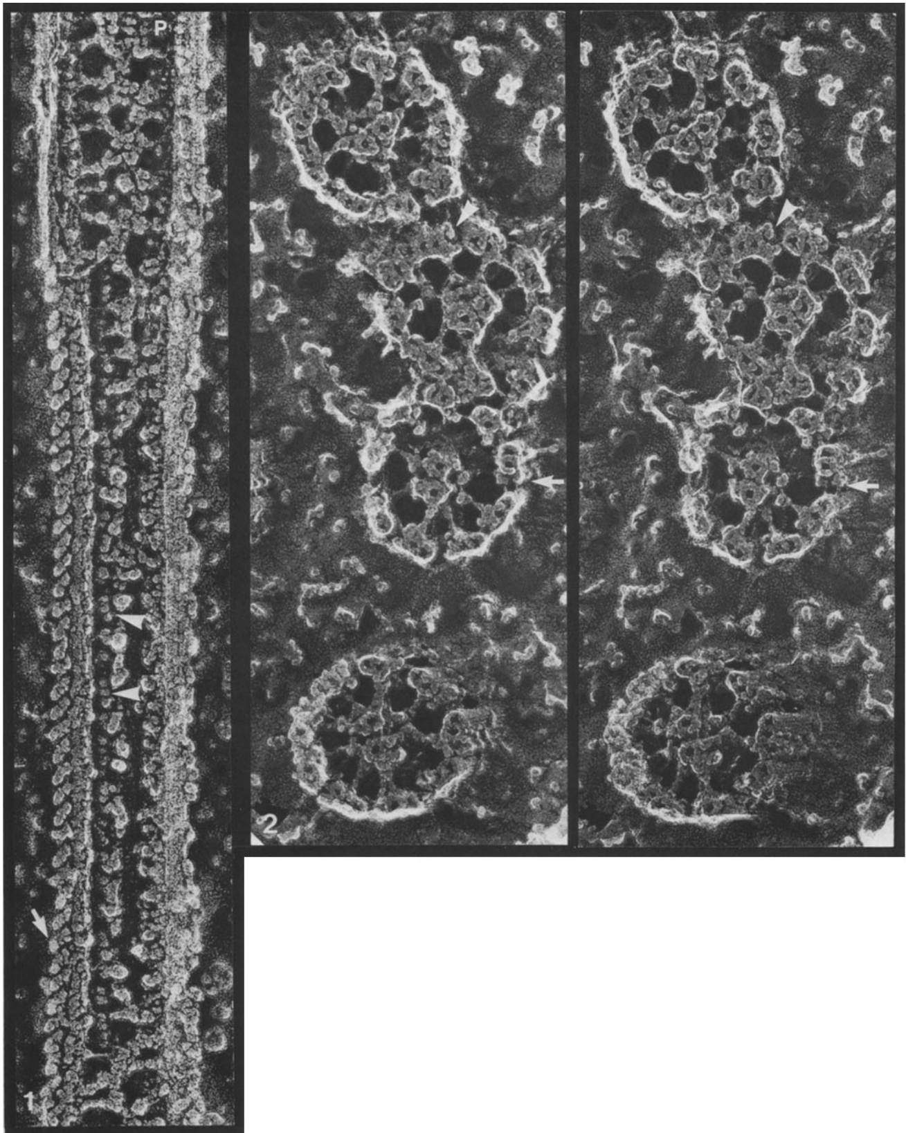
FIGURES 1 and 2 (Figure 1) Tetrahymena axoneme (rigor) in longitudinal fracture. A row of outer dynein arms on the left A microtubule is seen from the vantage point of the next B microtubule; we interpret the prominent head (arrow) on each arm to represent the third head which cannot be seen from the axoneme exterior and which creates the "hook" seen in cross section (discussed in reference 10). Clusters of deep inner arm heads are indicated by arrowheads. Longitudinal views of the radial spoke system are included at the top and bottom of the field; cross-fractured spokes appear in the center of the field as groups of irregular white objects. Central-pair projections at P. \times 185,000 . (Figure 2) Tetrahymena cilia in cross fracture, stereo pair, from a detergent-extracted cell. The radial spokes associate with the projections which stand up above and below the central pair and associate closely with the sides of the central pair. The helical disposition of the spokes is evident in stereo. Connections between the central-pair microtubules are visible in the bottommost axoneme. Arrow points to a well-preserved set of outer and inner arms showing their stalk connections to the B tubule; arrowhead indicates an outer arm with a prominent "hook." \times 165,000 .
