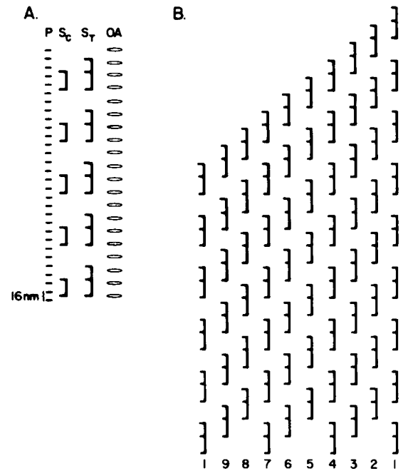
FIGURE 12 (A) Diagram of the spatial relationships between the central-pair projections ( P ), the spoke systems of Chlamydomonas ( S_c ) and Tetrahymena ( S_t ), and the outer arms ( OA ). (B) Diagram of the three-start right-handed helix formed by the radial spoke system in Tetrahymena . Spoke S_3 is absent from the otherwise equivalent system of Chlamydomonas .
