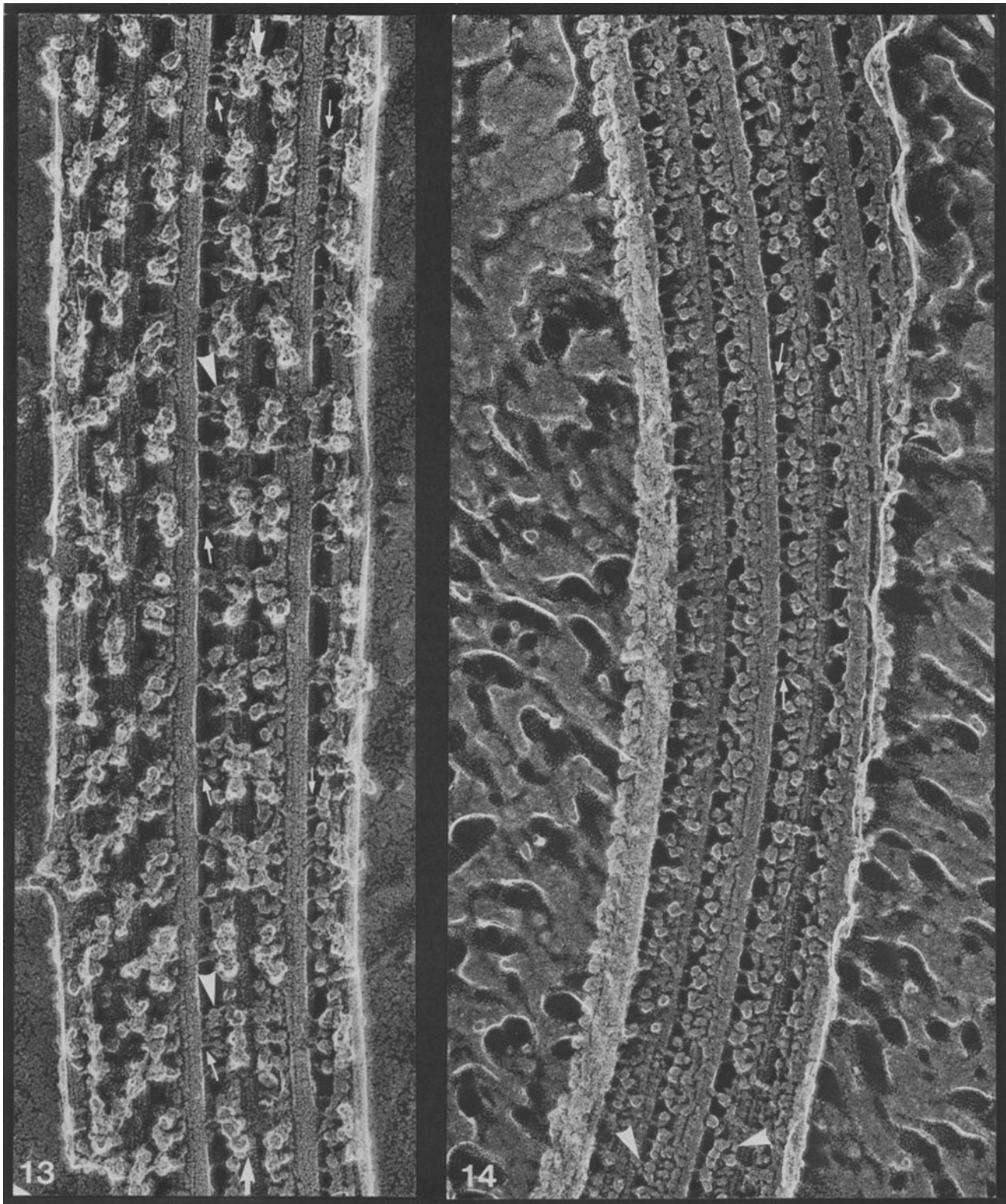
FIGURES 13 and 14 (Figure 13) Opened-out Tetrahymena axoneme subjected to overnight dialysis against Tris-EDTA (20). Large arrows mark doublet displaying optimal clusters of inner arms; these attach to the adjacent B tubule by slender stalks (small arrows) and associate with the A tubule via bulky domains (arrowheads). Radial spokes, fractured near their heads, appear as white clusters along the A tubules. Note that the helical alignment between sets of radial spokes (cf. Fig. 12) is preserved along the leftward three doublets, whereas the spokes are aligned in register along the rightward three doublets, an example of the shift in spoke alignment that accompanies shifts in doublet alignment (the shift here presumably accompanying or the consequence of the "opening-out" event). \times 125,000 . (Figure 14) Opened-out Chlamydomonas axoneme of the pf-14 strain lacking radial spokes. An optimal group of inner arm stalks attached to a B microtubule is marked by arrows; bulky domains associate with the rightward A tubule, and discrete globular heads lie in the interdoublet gap. Arrowheads point to distinct double-headed and triple-headed species. Row of outer arms is visible along the leftmost doublet (cf. Fig. 1). \times 140,000 .
