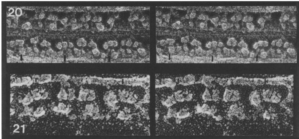
FIGURES 20 and 21 Stereo views of Chlamydomonas inner arms in rigor axonemes. Triad positions are indicated by bars. (Figure 20) pf-14 mutant. \times 230,000 . (Figure 21) Wild-type. \times 390,000 .
