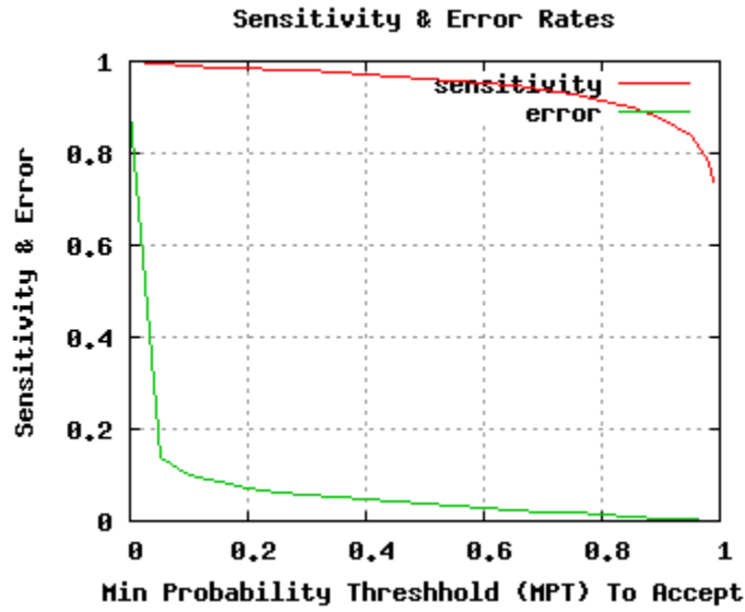
Plasma GPF8: sensitivity & error rates plot
