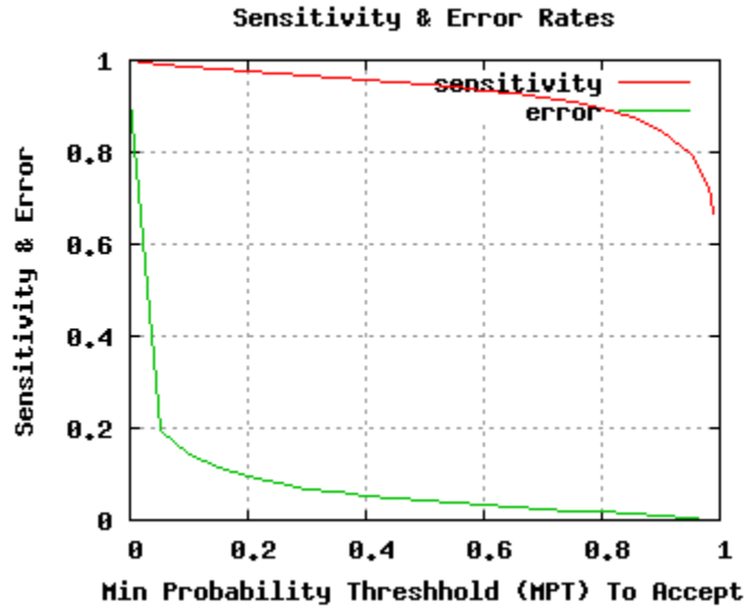
Plasma PACIFIC: sensitivity & error rates plot
