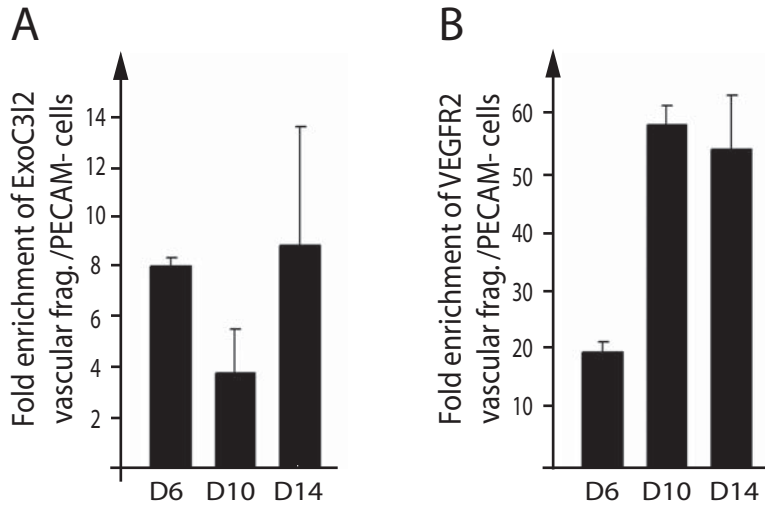
Supplemental Figure 2. Expression of exoc3l2 mRNA at different time points in the EB cultures. (A) Endothelial cells were extracted from VEGFA-stimulated EBs using magnetic beads and the expression of exoc3l2 was measured after 6, 10 and 14 days in culture. The results were compared to the expression in the PECAM - cells. (B) The expression of VEGFR2 in the endothelial cell population, compared to PECAM - , after 6, 10 and 14 days in culture.
