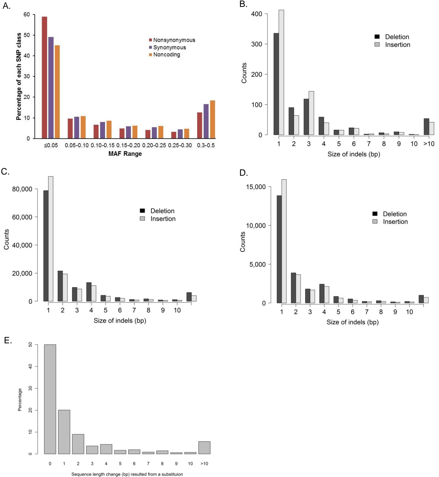
Figure S3. SNP allele frequency and size distributions of indels and block substitutions. A , Fraction of nonsynonymous, synonymous, and noncoding SNPs in each minor allele frequency (MAF) class. B-D , Size distribution of indels in B ) coding regions, C ) introns, and D ) UTRs, respectively. E , Distribution of change in sequence length caused by block substitutions.
