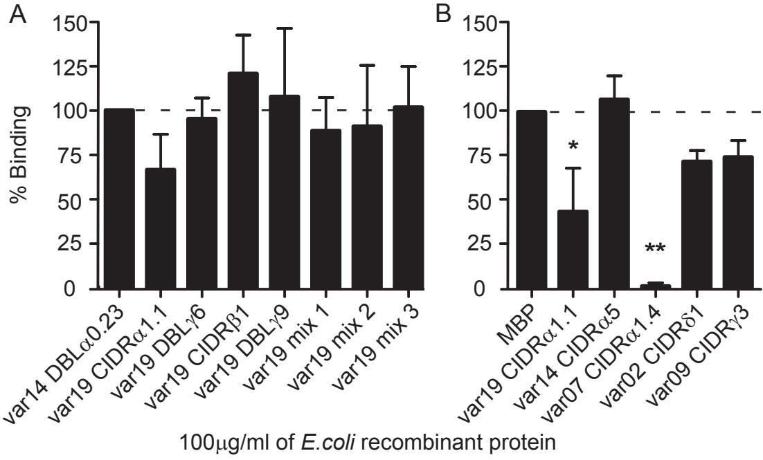
Figure S4. DC8 and DC13 CIDR1 domains inhibit DC8-IE binding to THBMEC.
