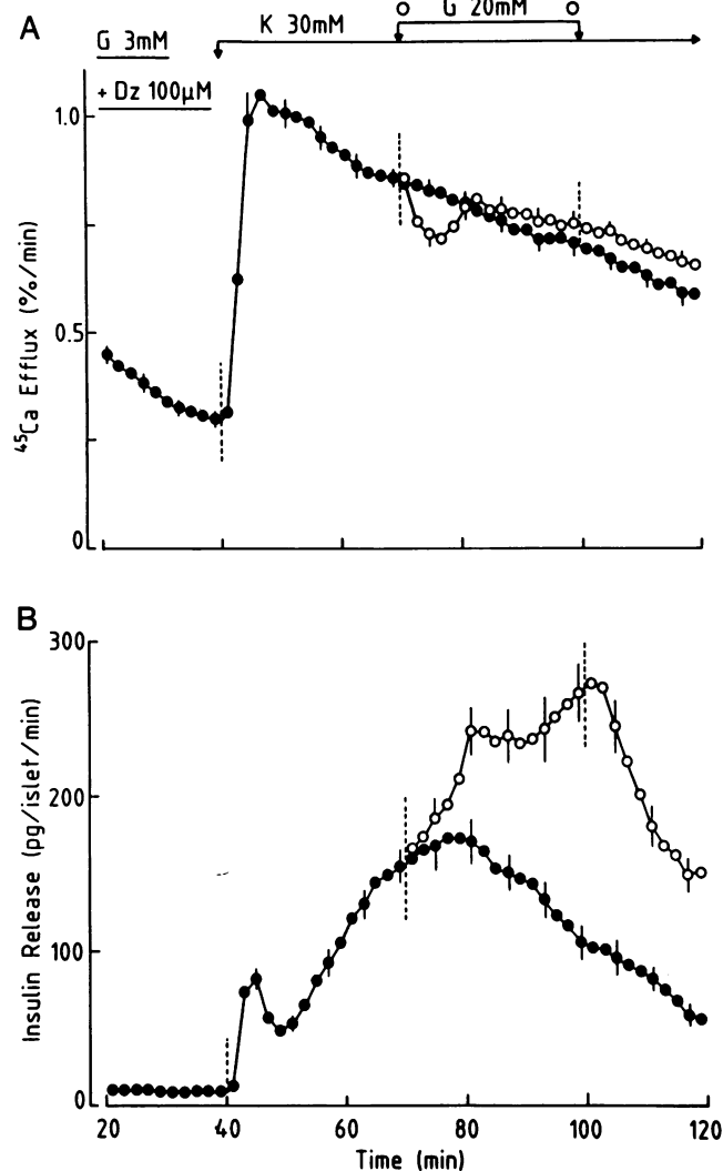
Figure 5. Effects of glucose on the stimulation of ^{45}\text{Ca} efflux and insulin release by 30 mM K in mouse islets perfused with a medium containing 100 \mu M diazoxide (Dz) throughout. The experiments were started with a medium containing 3 mM glucose (G) and 4.8 mM K. The concentration of K was then increased to 30 mM from 40 min. In one series (○—○), the concentration of glucose was increased to 20 mM between 70 and 100 min. Values are mean \pm SEM for six parallel experiments.
