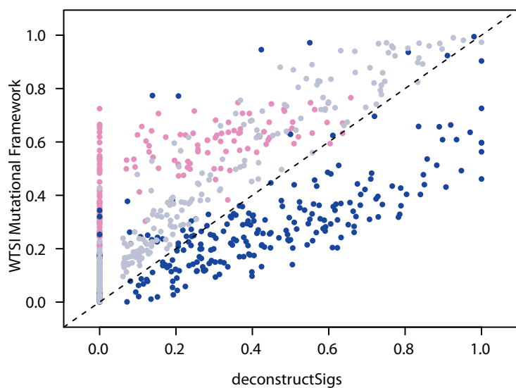
LUAD comparison
