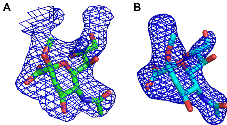
S3 Fig. Simulated annealing omit (Fo-Fc) electron density maps of glycan ligands bound to H7 HA triple mutant. (A) LSTc bound to the triple mutant HA. (B) LSTa bound to the triple mutant HA. The electron density for the glycan receptors is represented in a blue mesh and contoured at 2.5 \sigma .
