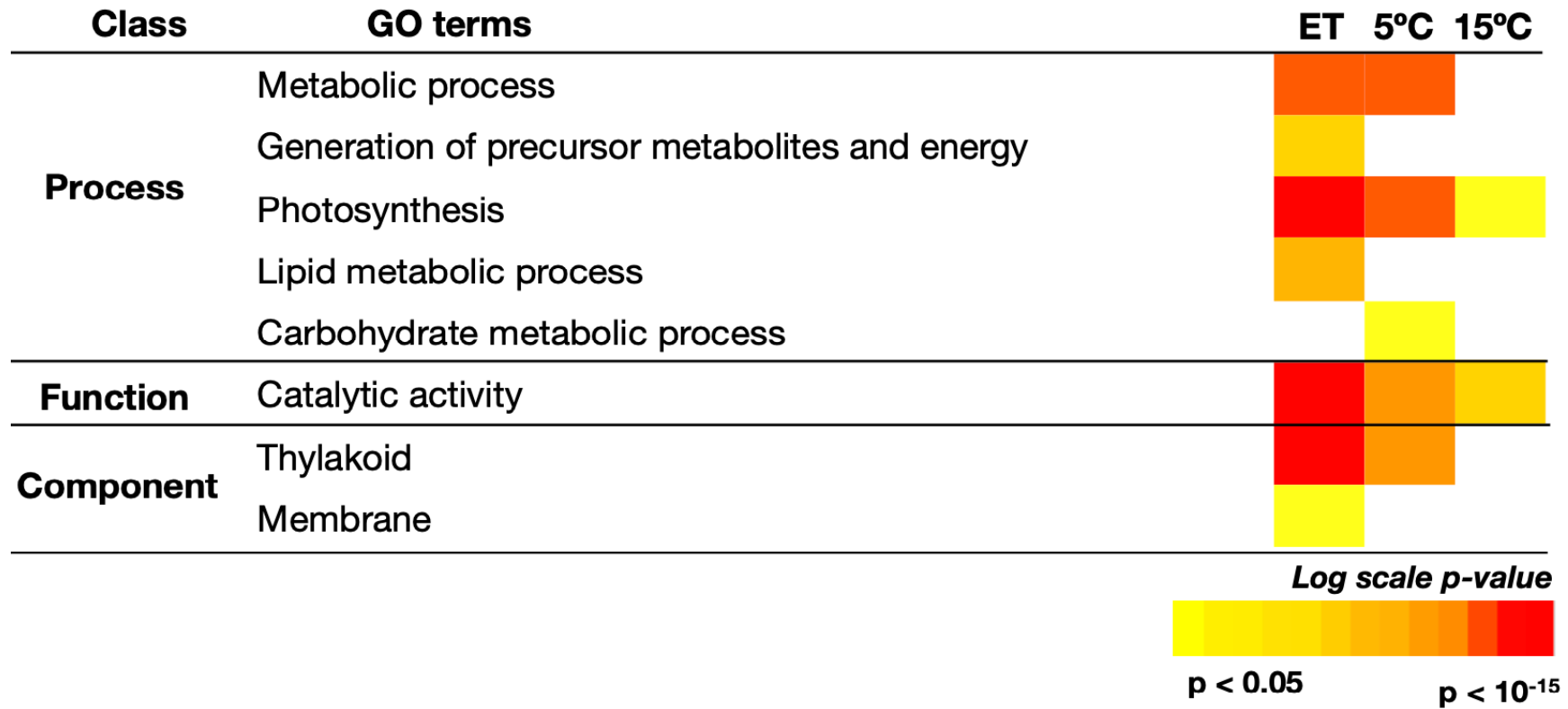
Fig. S2. Selected GO terms enriched among the DEGs identified in lemon fruit exposed to ethylene, 5°C and 15°C.
