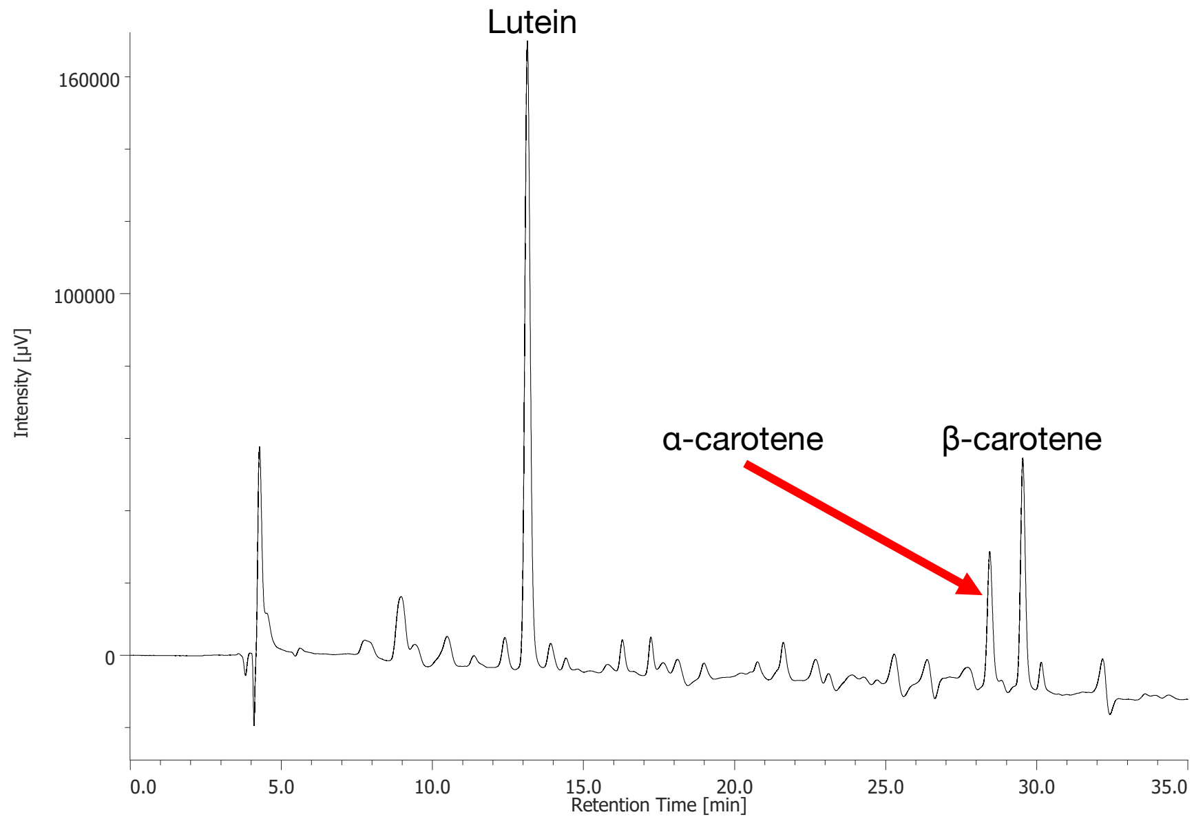
Fig. S1. Chromatogram showing the major carotenoid pigments identified in the flavedo of lemom fruit.
