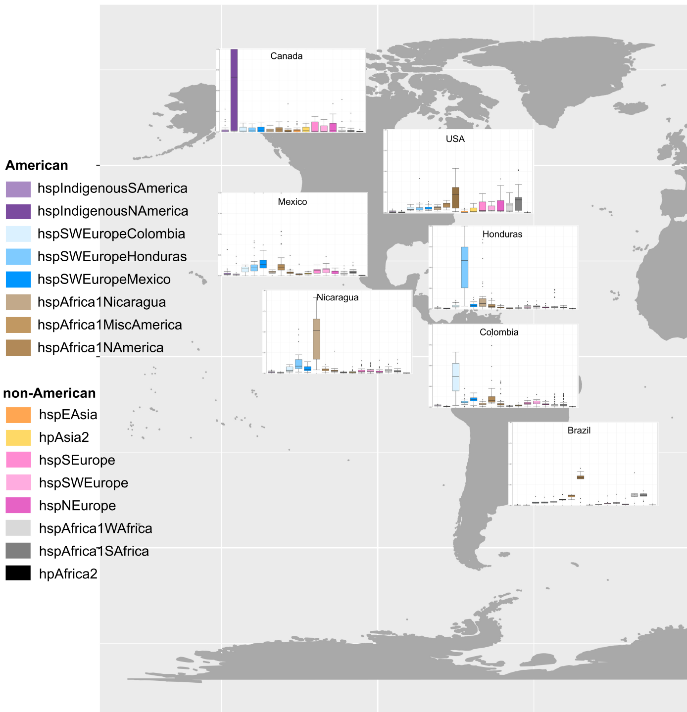
Suppl. Fig 3. Comparative admixture analyses of H. pylori strains in the Americas by country.
