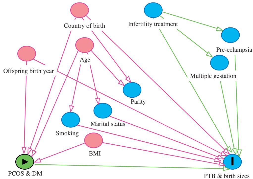
Supplementary Figure S1. Directed acyclic graph derived from previous literature and expert knowledge. Nodes represent ancestors of exposures and/or outcomes, and lines indicate biasing or causal paths. Exposures are PCOS (polycystic ovary syndrome) and comorbid diabetes mellitus (DM), and outcome measures include preterm birth (PTB) and birth sizes (large or small for gestational age).
