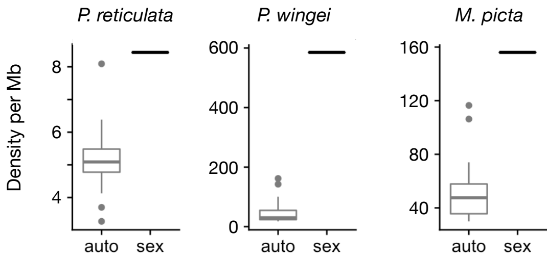
Supplementary figure S1. Densities of SDR-like SNPs on sex chromosomes and autosomes.
