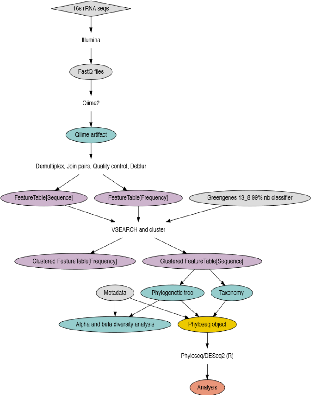
Fig. S1 Data processing and analysis pipeline for Saudi T2D 16S microbiota study
