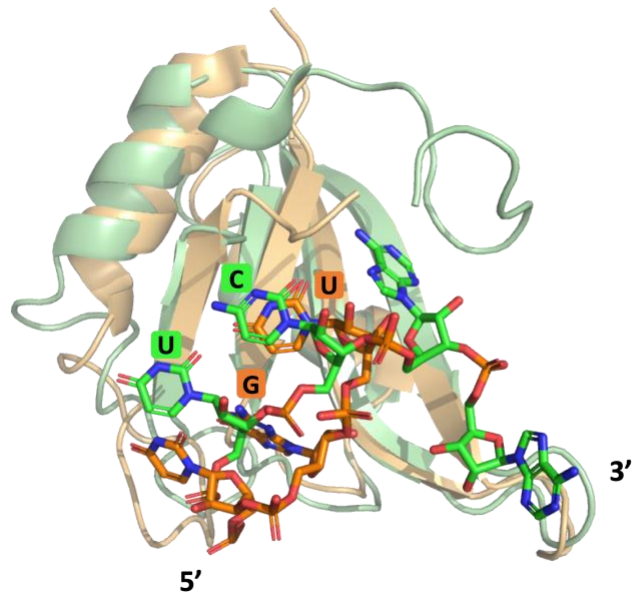
S3 Fig: Superimposed RRM-RNA complexes with the lowest similarity score in cluster 0, PDB Id. 6g90 (chain B, green) and PDB Id. 3nh (chain B, orange). The aligned nucleotides used for the RMSD calculations are labelled.
