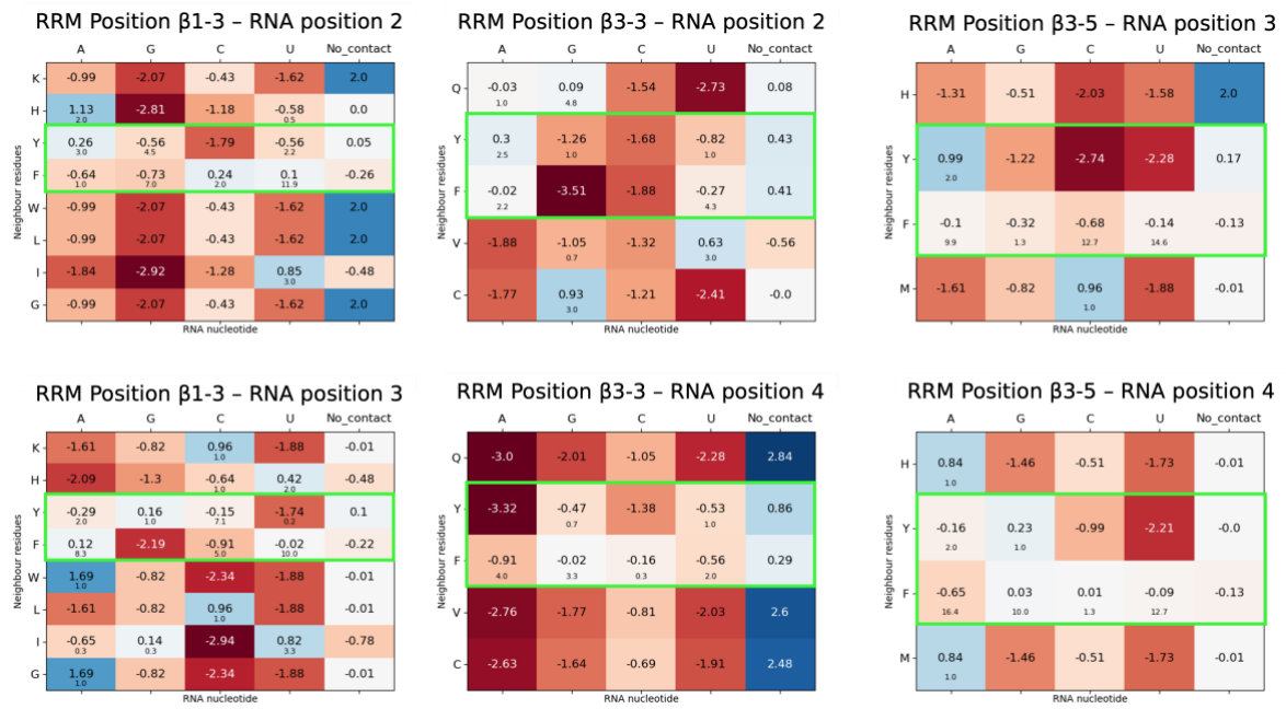
S4 Fig: Scores for the conserved aromatic positions in RNP1 ( \beta 1-3) and RNP2 ( \beta 3-3, \beta 3-5) in contact with their respective RNA positions (phenylalanine and tyrosine scores are highlighted in bright green).
