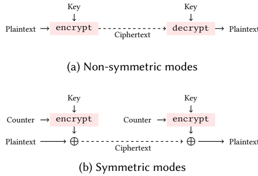
Fig. 1. Operations in two types of block cipher modes
