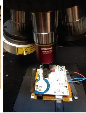
(c) LASER fault injection on a microcontroller
