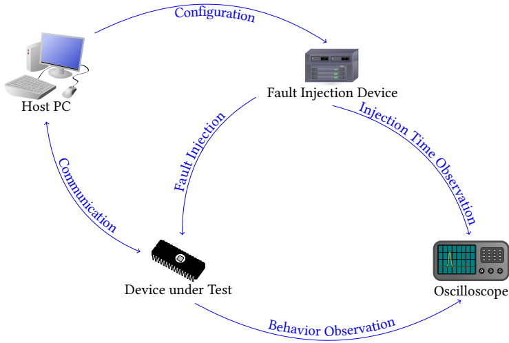
Fig. 3. Schematic view of a fault injection set-up
