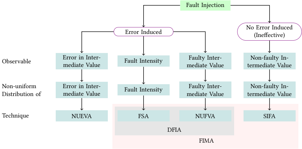
Fig. 9. Overview of statistics based fault analysis methods
