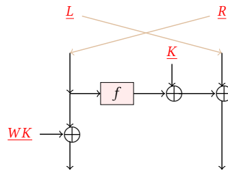
Fig. 7. Last round of many Feistel network based ciphers
