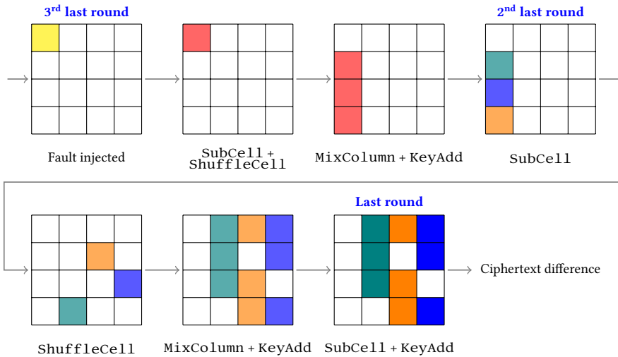
Fig. 6. DFA on MIDORI encryption at third last round
