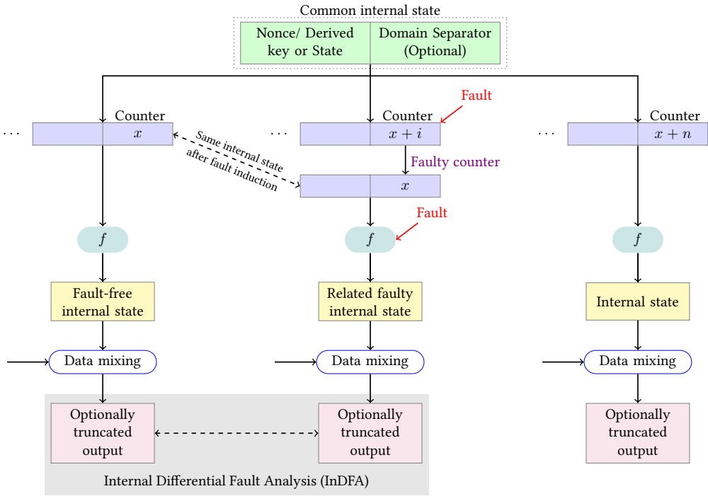
Fig. 8. Generic model for using internal differentials in fault analysis of parallelizable ciphers in the counter mode
