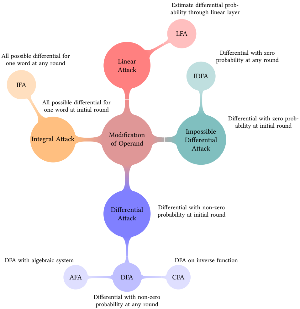
Fig. 2. Attacks (classical and fault) based on modification of operand models
