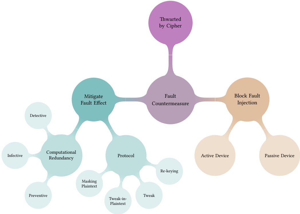
Fig. 10. Generic overview of fault attack countermeasures
