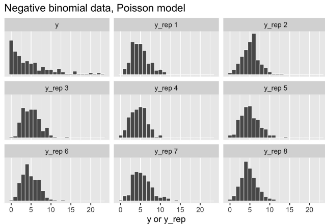
Figure 28.2: Posterior predictive checks for negative binomial data generating process and Poisson model.
