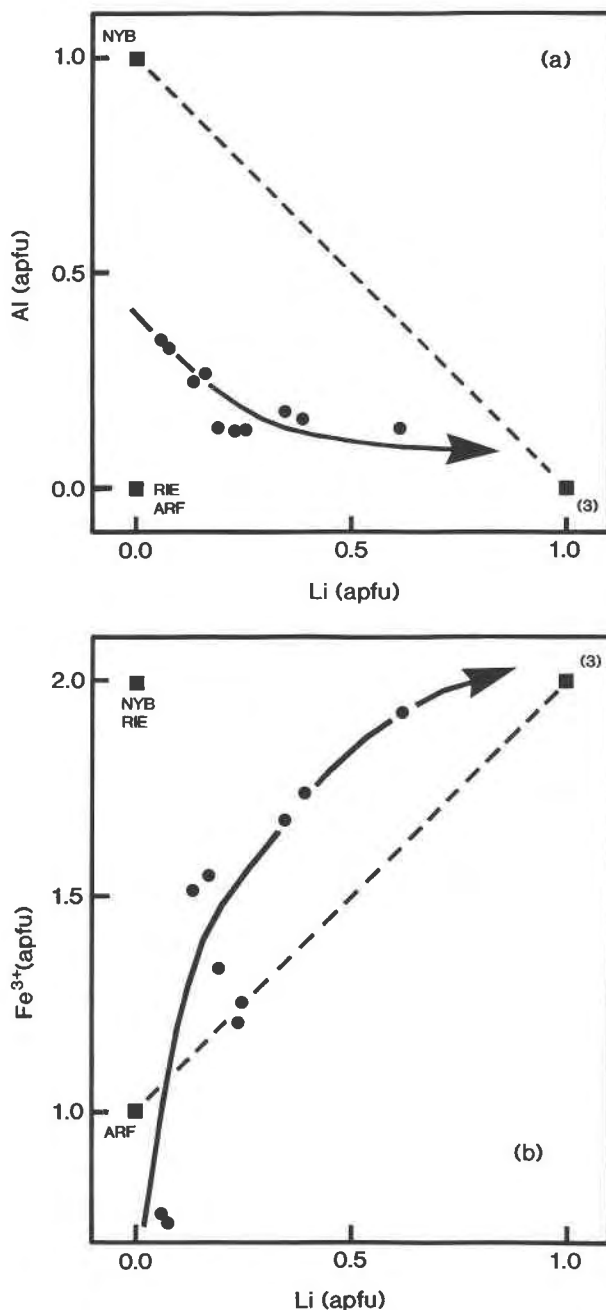
Fig. 7. (a) Variation in 141 Al as a function of Li content; (b) variation in Fe 3+ as a function of Li content. ARF = arfvedsonite, NYB = nyboite, RIE = riebeckite, (3) = end-member 3 from Table 9.
