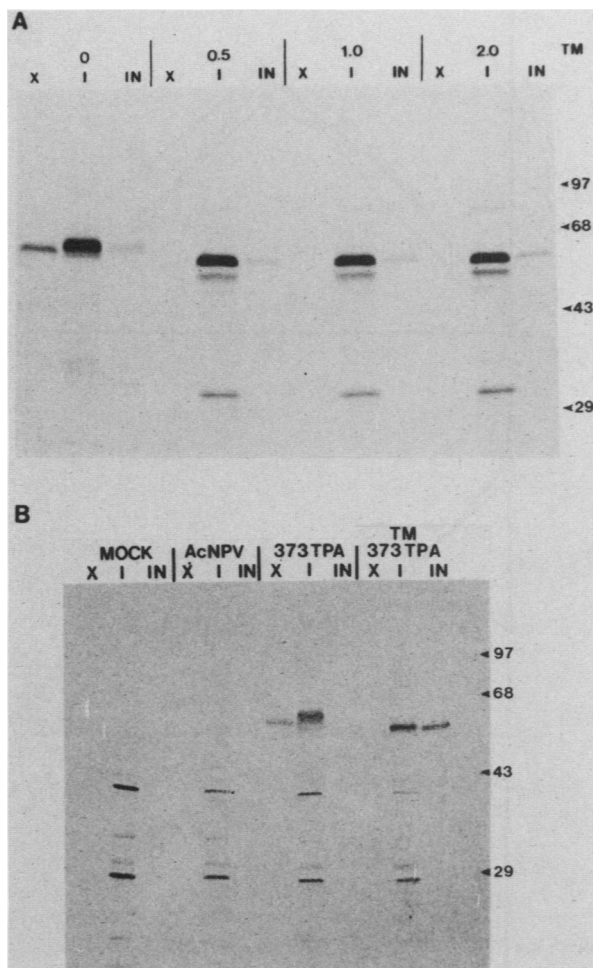
FIG. 5. Effect of TM treatment on t-PA secretion from Sf9 cells. (A) 373-t-PA-infected Sf9 cells were untreated (0) or treated for 8 h with 0.5, 1.0, or 2.0 \mu\text{g} of TM per ml, as indicated above the lanes. The cells were labeled with 100 \mu\text{Ci} of [ ^{35}\text{S} ]Translabel per ml from 20 to 24 hpi, corresponding to the last half of the TM treatment period. Extracellular (X), intracellular (I), and insoluble (IN) fractions were prepared, and t-PA was immunoprecipitated and analyzed by SDS-PAGE. (B) Cells were mock infected or infected with wild-type baculovirus (AcMNPV) or 373-t-PA and were untreated or treated with 1.0 \mu\text{g} of TM per ml, as indicated above the lanes. Extracellular (X), intracellular (I), and insoluble (IN) fractions were prepared, and proteins were resolved directly by SDS-PAGE and analyzed by Western transfer with goat anti-t-PA as the probe as described in Materials and Methods. Numbers at right are as in Fig. 1.
