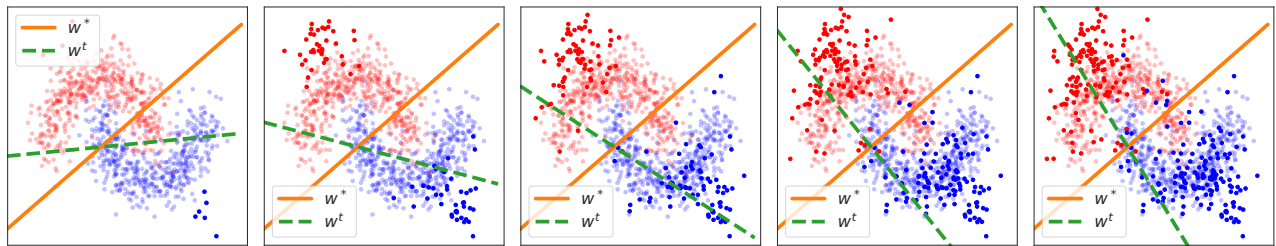
Figure 19: Visualization of the data synthesized by a VAE-based teacher after iteration 10, 80, 150, 240, and 290. The orange line indicates the target classifier w^* ; the green dashed line indicates the student classifier. Different colors indicate different classes; points with lower opacity represent the ground truth data distribution.
