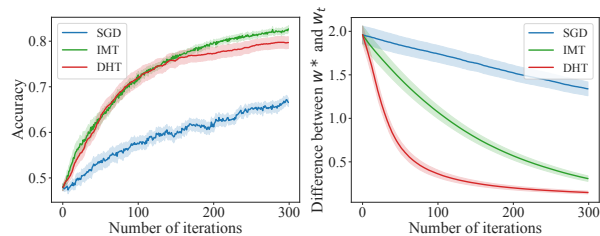
Figure 9: Convergence of privacy-preserving teaching on MNIST.
