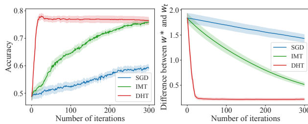
Figure 24: Accuracy and weight convergence using parametrized black-box teaching policy in 3/5 classification on MNIST.
