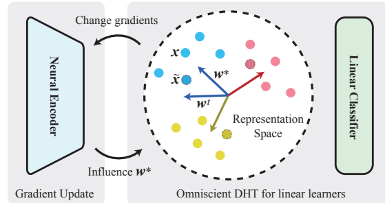
Figure 2: Performative teaching for black-box neural learners.
