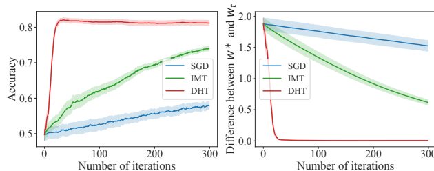
Figure 14: Accuracy and weight convergence using data transformation policy in 3/5 classification on MNIST.
