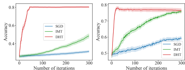
Figure 8: Convergence of black-box parameterized teaching policy with the full teaching space. Left: half-moon. Right: MNIST.
