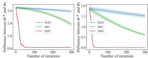
Figure 4: Convergence of data transformation policy. Left: binary classification on half-moon. Right: 3/5 classification on MNIST.
