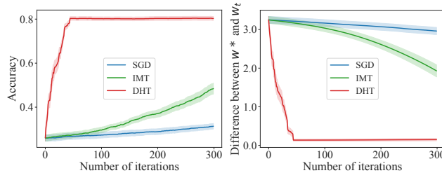
Figure 23: Accuracy and weight convergence using parametrized black-box teaching policy in binary classification on half-moon.
