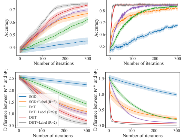
Figure 3: Omniscient teaching with or without label synthesis [14]. Convergence comparison between our greedy teaching policy with several other baseline methods. Left: half-moon. Right: MNIST.
