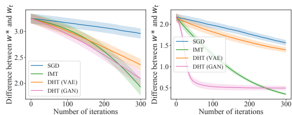
Figure 5: Convergence of GAN-based and VAE-based generative modeling policy. Left: half-moon. Right: MNIST.
