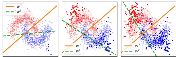
Figure 6: Visualization of the data synthesized by a VAE-based teacher after iterations 10, 150, and 290. The orange line indicates the target classifier w^* ; the green dashed line indicates the student classifier. Different colors indicate different classes; points with lower opacity represent the ground truth data distribution.
