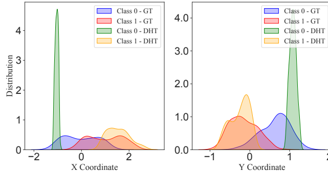
Figure 18: Visualization of the data distribution of the synthesized data by a GAN-based teacher after 300 iterations. GT denotes the ground truth.
