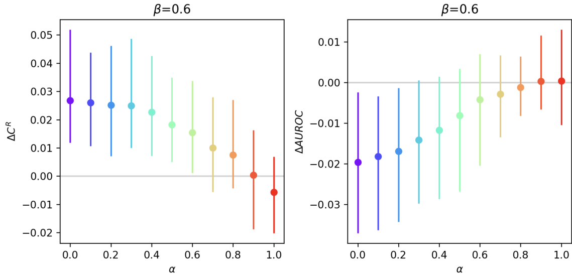
Figure 7: Performance Difference for \beta = 0.6 Sweeping Across \alpha . Comparing \Delta \mathcal{C}^R and \Delta \text{AUROC} for various \alpha values. In this case see a more limited benefit of the “RBC models” over “BCE models”, with \alpha \in [0.3, 0.6] showing significant benefit in \mathcal{C}^R and no significant degradation in AUROC.
