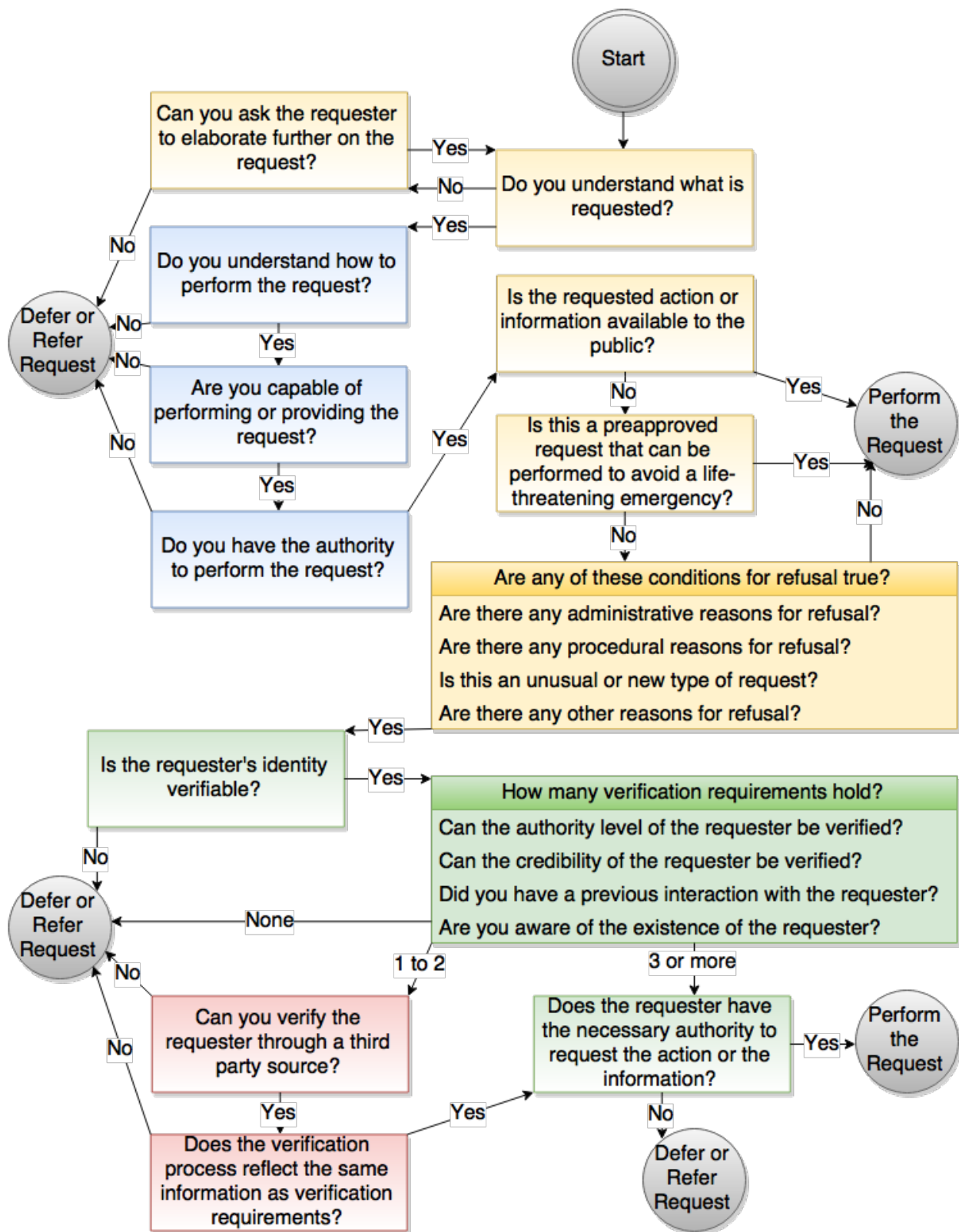
Figure 3: Social Engineering Attack Detection Model [60]
