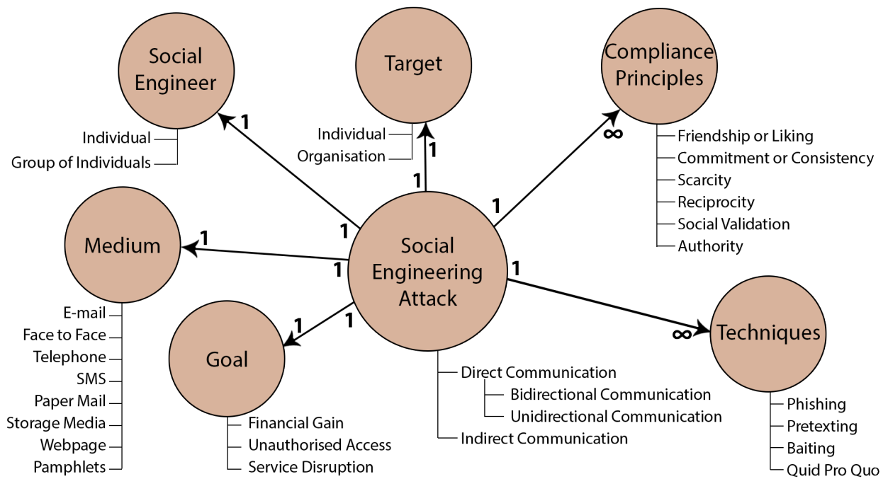
Figure 1: An ontological model of a social engineering attack
