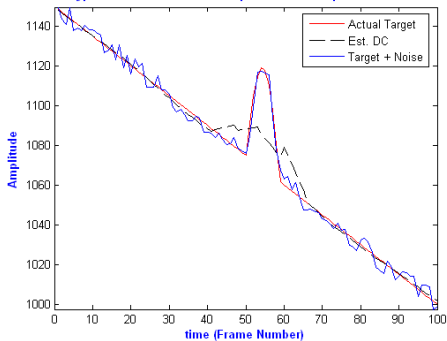
Type 3 SNR=4 VarWin= 4 GroupWin= 15 Overlap= 5 DCWin= 20
