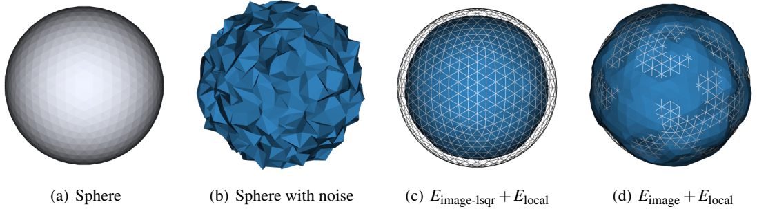
Figure 5.4.: A sphere (a) is modified by randomly displacing points along their surface normals (b), which simulates deformation caused by the ASM’s image feature search. The deformed sphere defines the vector \hat{\boldsymbol{x}} . (c): If an optimization is started that combines the local energy with the least squares image energy, E_{\text{image-lsq}}(\boldsymbol{x}; \hat{\boldsymbol{x}}; \boldsymbol{w}) , the optimized shape is considerably smaller than the original sphere. (d): If E_{\text{image}}(\boldsymbol{x}; \hat{\boldsymbol{x}}; \boldsymbol{w}) is used as image force, the scale is maintained.
