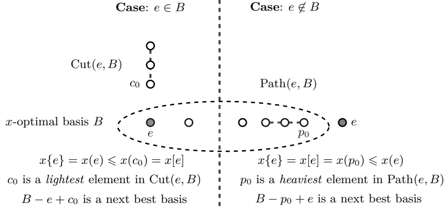
FIGURE 1. A schematic summary of Lemma 1. A lightest (resp., heaviest ) element of a set S \subseteq E is an element of S of the minimum (resp., maximum) weight (there may be several such elements). If e \in B , then a next best basis is a basis which has the minimal weight under all bases avoiding the element e . If e \notin B , then a next best basis is a basis which has the minimal weight under all bases containing the element e .
