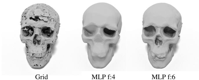
Figure 26. Comparing grid vs. MLP parametrizations of DMTet on scan 65 from the DTU MVS dataset [28]. Directly optimizing SDF values at grid vertices leads to a surface with high-frequency noise (left). In contrast, if we use an MLP to parametrize the SDF values, we can regularize the geometry, with smoothness controlled by the frequency of positional encoding. We use the positional encoding in NeRF [45] with frequency set to 4 (middle) and 6 (right) respectively.
