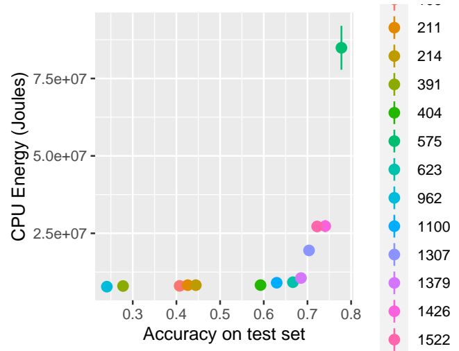
Fig. 6. Pareto Front: MLP on the Glass data set. The trade-off of model accuracy on test data vs CPU energy for inference.
